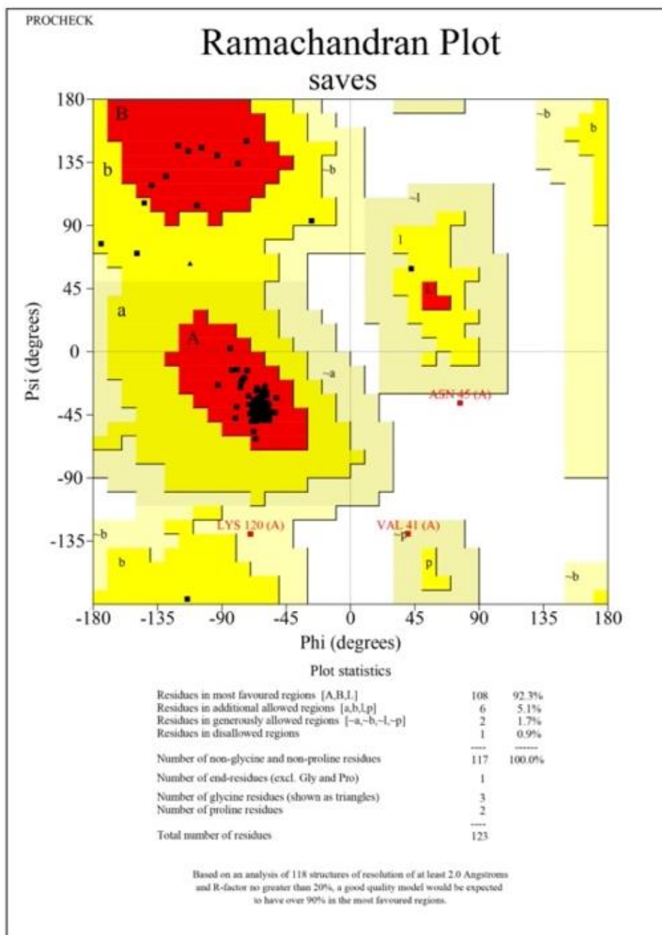
Figure S4. Ramachandran plot of the predicted KCNE2 protein structure generated using PROCHECK (SAVES v6.1). The majority of residues are located in favored and allowed regions (92.3%), indicating acceptable stereochemical quality and overall geometric plausibility of the predicted model.
